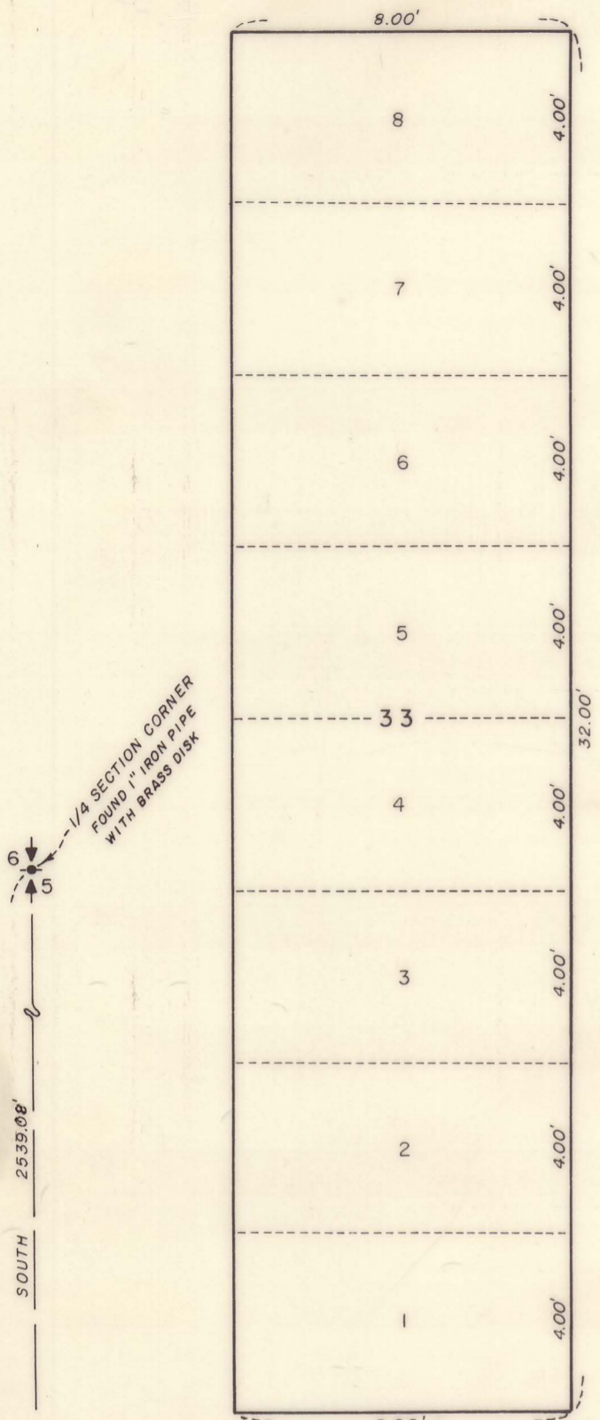
TYPICAL PLOT PLAN BLOCK NO. 3 SCALE: 1" = 4.00'
