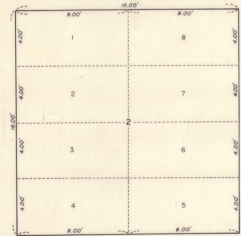
TYPICAL PLOT PLAN BLOCK NO. 1 & 2 SCALE: 1" = 4.00'
