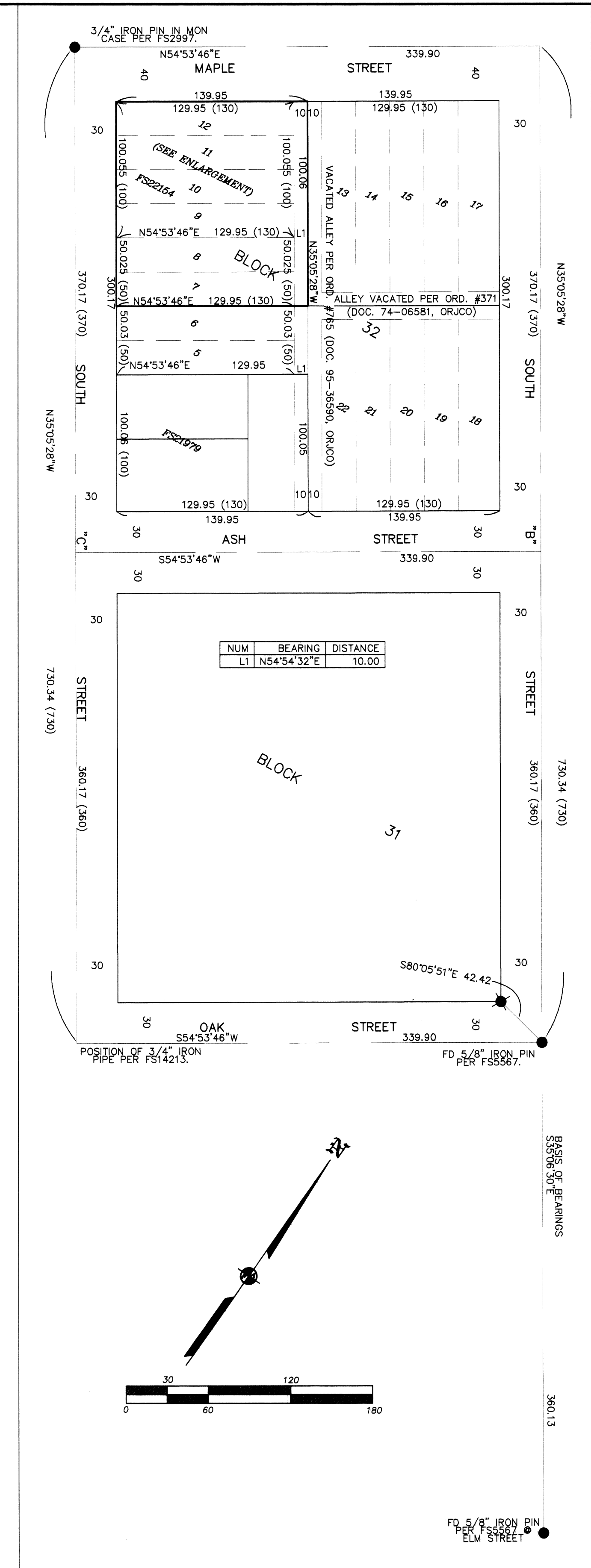
OVERALL MAP - 1"=60'
